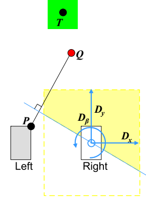
Fig. 6. In this figure the allowable stepping zone is shown in yellow. The left foot is the support foot. P is the CoP with the single support and Q is the reference point. The allowable stepping zone is the upper part of the rectangle (above the blue separatrix) with edges D_x and D_y . D_\beta denotes amount of rotation of the swing foot.
