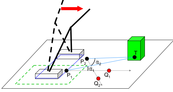
Fig. 5. Schematic of a biped robot subject to a fall. P_1 is the current CoP, and Q_1 is the reference point when the controller starts, and the robot will fall in the direction P_1Q_1 . T is the target to avoid. The support base is shown in blue dotted lines. The green dotted lines enclose the allowable stepping zone, the region where a new CoP can be placed through proper foot placement. P_2 is a candidate for the new CoP by stepping. Q_2 is the estimated new reference point when the step is taken. \alpha_i is the avoidance angle between P_iQ_i and P_iT . The fall controller will try to maximize \alpha_2 .
